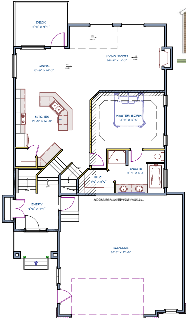
MAIN FLR.
